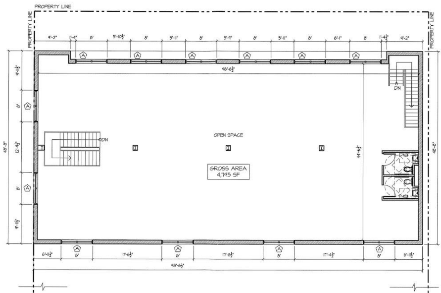
1 PROPOSED NEW SECOND FLOOR Scale: 3/32"=1'-0"
