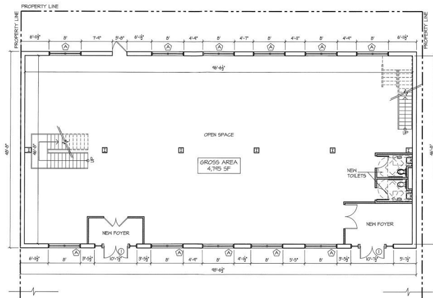
1 PROPOSED FIRST FLOOR Scale: 3/32"=1'-0"
